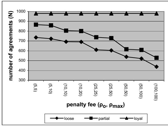
Figure 2: Number of successful negotiations for varying penalty fee.
