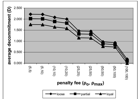
Figure 4: Number of buyer's decommitments for varying penalty fee.
