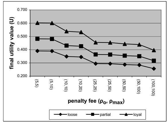
Figure 3: Final utility value for varying penalty fee.
