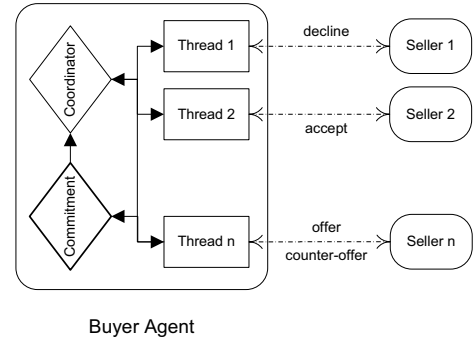
Figure 1: System architecture.
