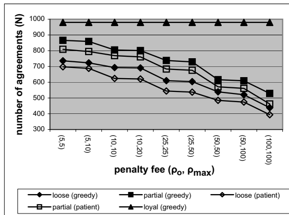
Figure 6: Number of successful negotiations for varying penalty fee.
