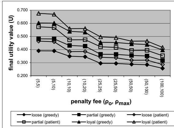
Figure 5: Final utility value for varying penalty fee.
